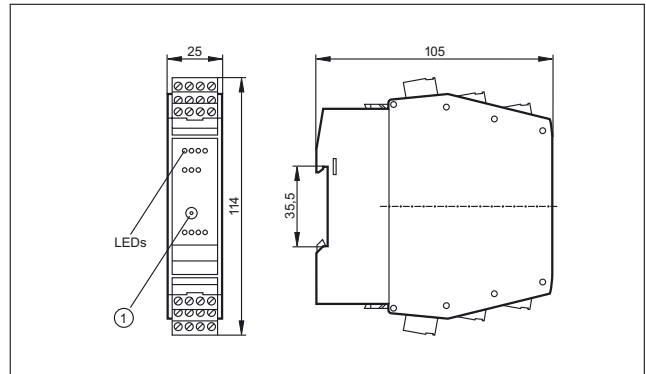
1: Addressing socket
