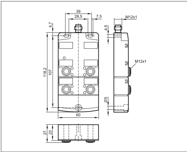
1: Addressing socket
