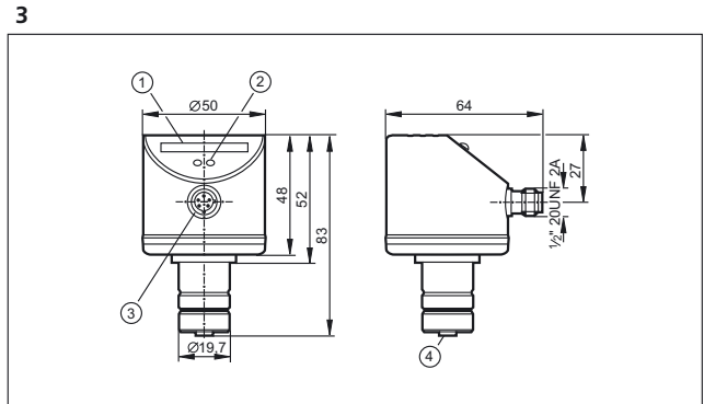
1: LED display, 2: setting pushbutton, 3: connection for voltage supply and output signals, 4: connection for flow sensor
