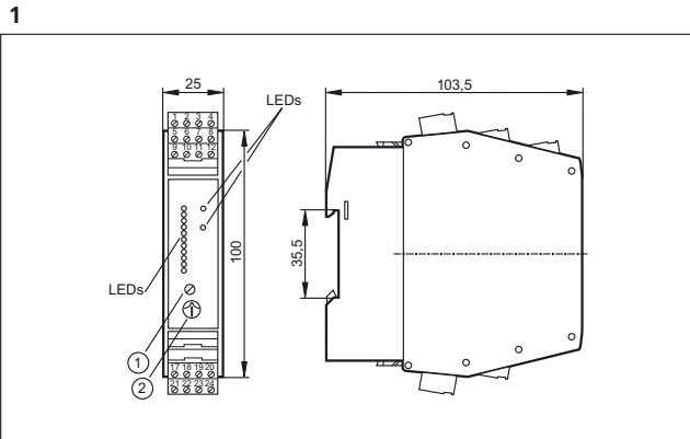
1: Potentiometer (switch point flow), 2: Potentiometer (switch point temperature)
