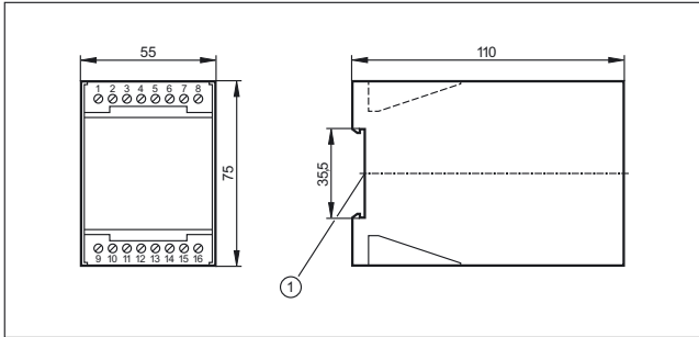
1: Mounting on DIN rail
