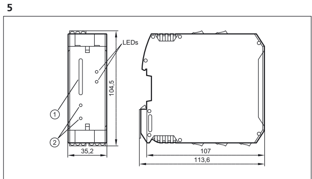
1: LED display, 2: setting pushbuttons
