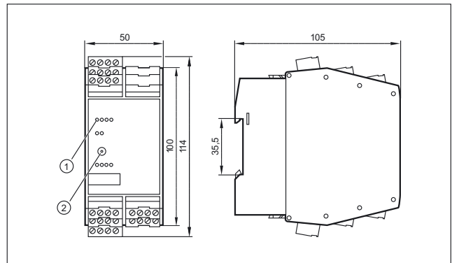
1: LED, 2: Addressing socket
