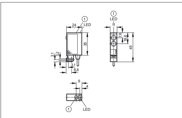
1: pushbutton
