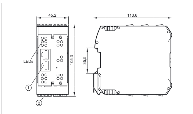
1: Ethernet interface, 2: screw terminals
