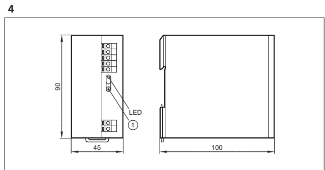
1: potentiometer
